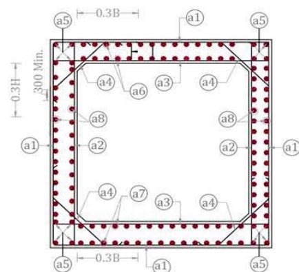
REINFORCEMENT DETAILS OF BOX CULVERT
