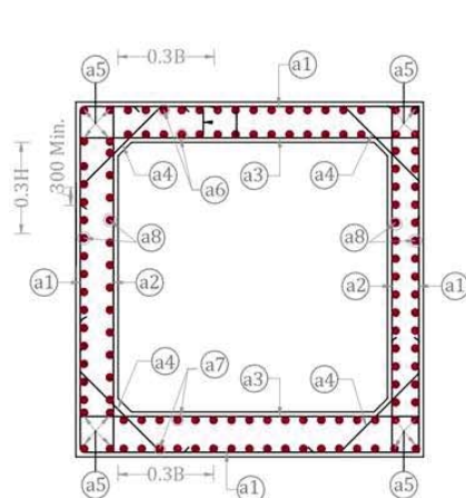
REINFORCEMENT DETAILS OF BOX CULVERT
