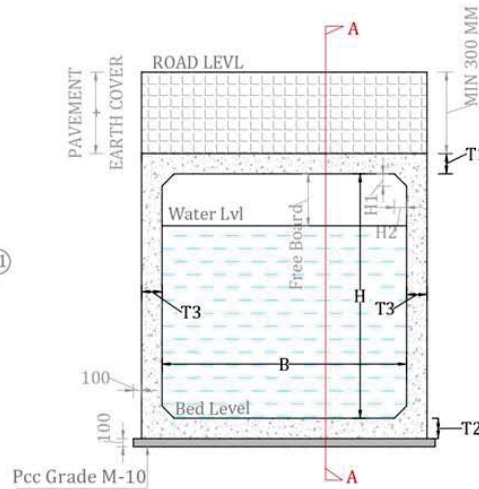
TYPICAL CROSS SECTION OF BOX SEGMENT
