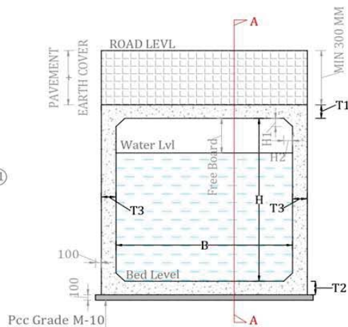
TYPICAL CROSS SECTION OF BOX SEGMENT
