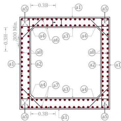
REINFORCEMENT DETAILS OF BOX CULVERT
