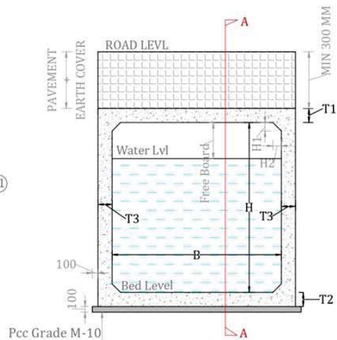
TYPICAL CROSS SECTION OF BOX SEGMENT
