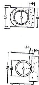
PLAIN CEMENT CONCRETE CRADLE BED AND ENCASING OF RCC PIPES
