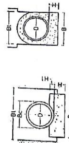
PLAIN CEMENT CONCRETE CRADLE BED AND ENCASING OF RCC PIPES
