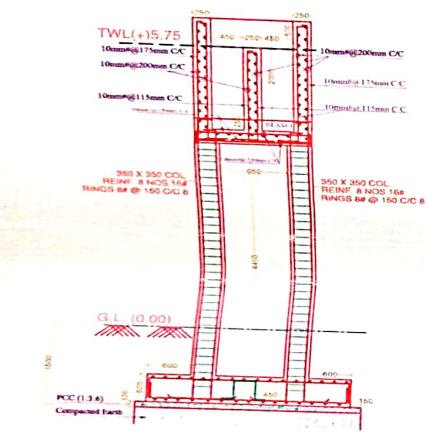
SECTION AT B-B
