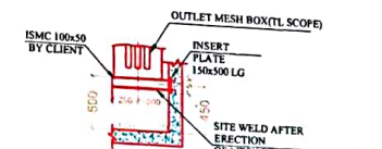
DETAIL 'Y' AT 2 PLACES
