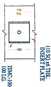
TYP INSERT PLATE DETAIL WITH CHANNEL FOR PUMP MOUNTING
