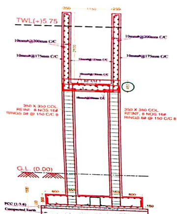
SECTION AT C-C
