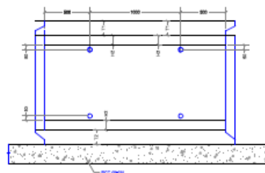
TOP PLAN SHOWING POSITION OF LIFTING HOLES
