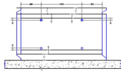
TOP PLAN SHOWING POSITION OF LIFTING HOLES
