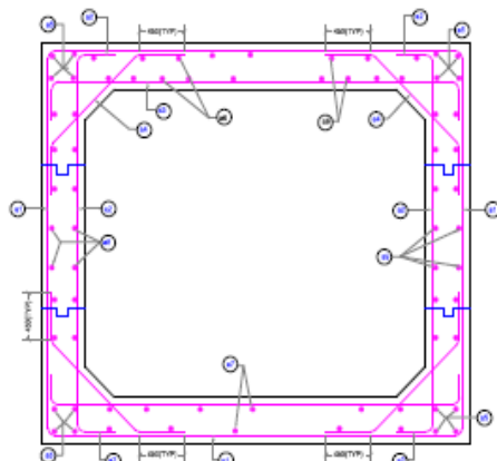
REINFORCEMENT DETAILS OF RCC SINGLE CELL BOX CULVERT
