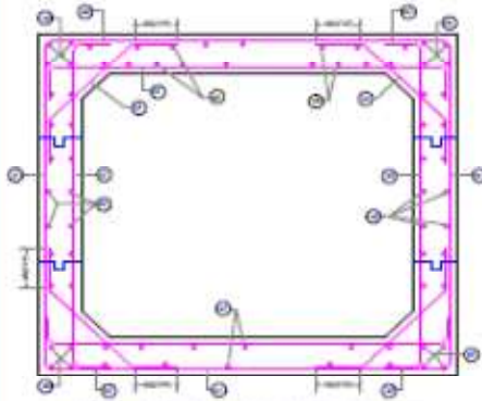
REINFORCEMENT DETAILS OF RCC SINGLE CELL BOX CULVERT
