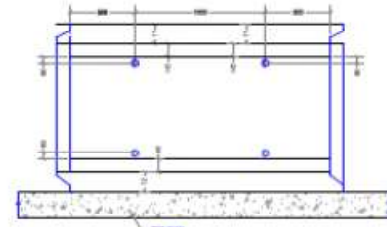
TOP PLAN SHOWING POSITIONS OF LIFTING HOLES
